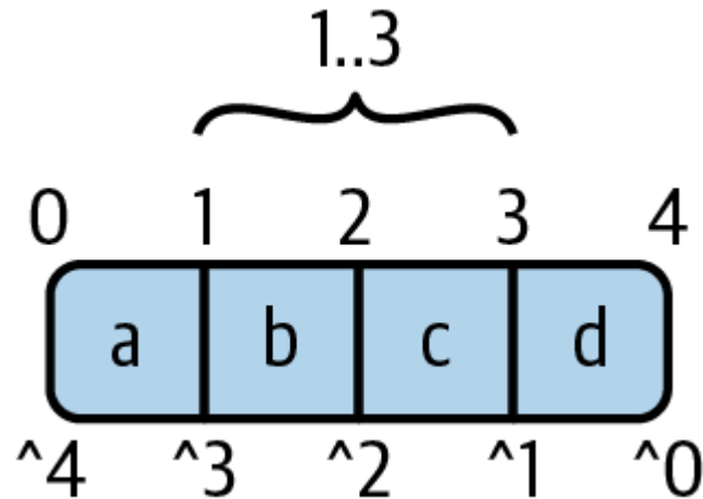
Figure 5-2. A range
