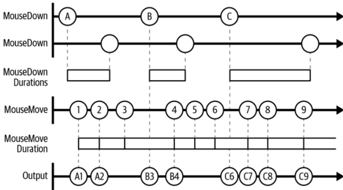
Figure 11-6. Join operator
