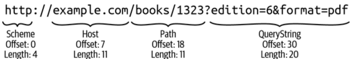
Figure 18-1. URL substrings
