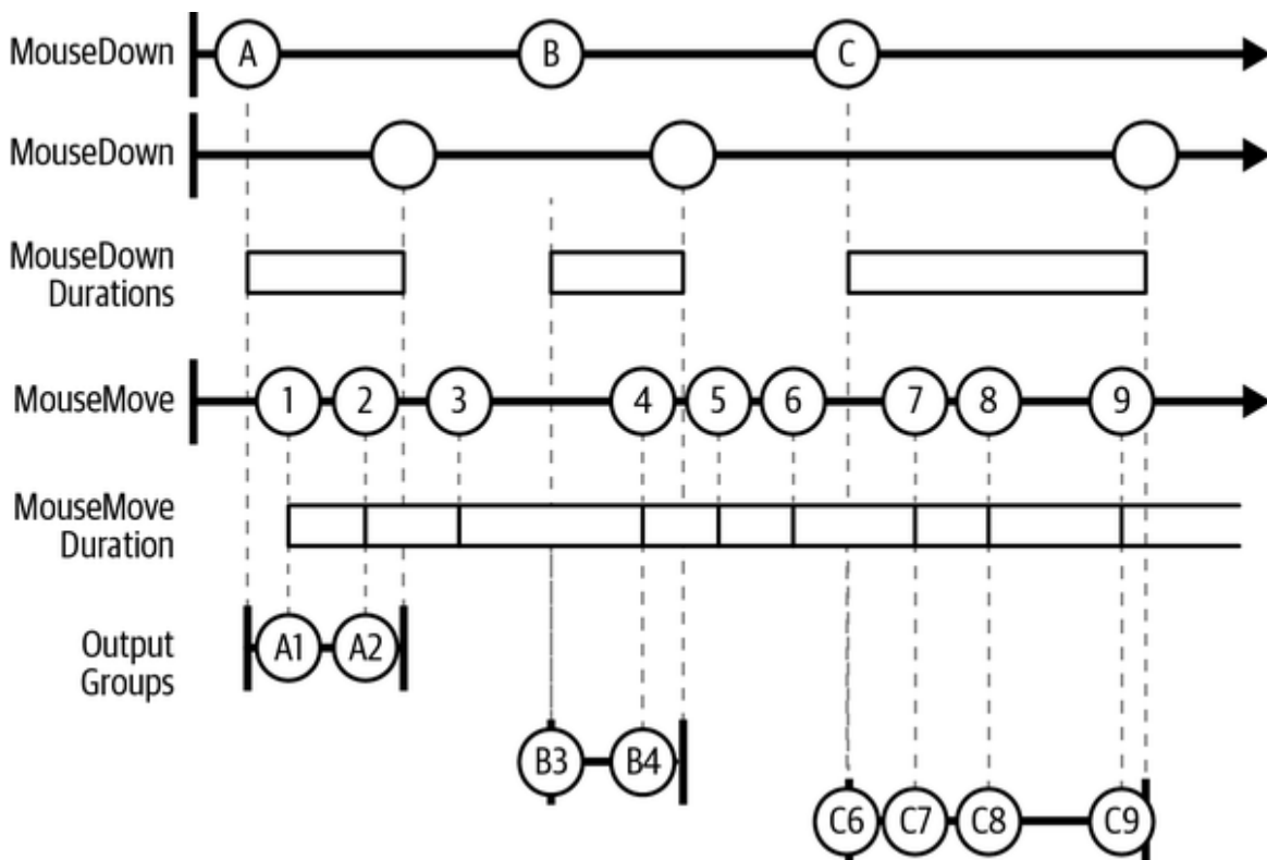
Figure 11-7. GroupJoin operator
