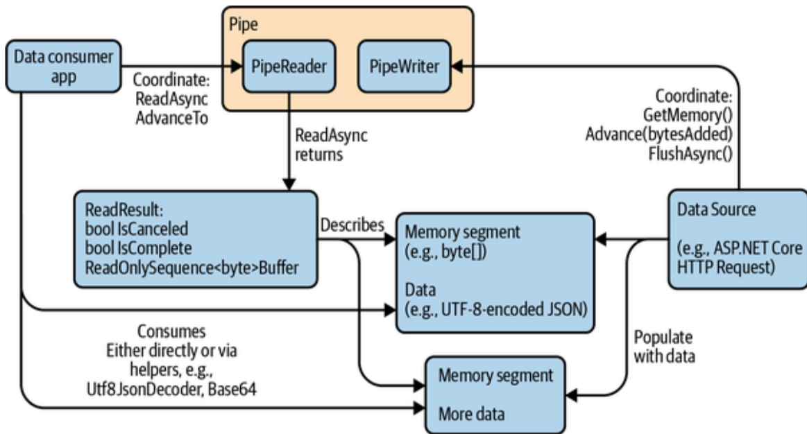
Figure 18-2. Pipeline overview
