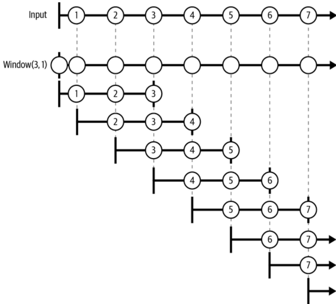
Figure 11-10. Window operator
